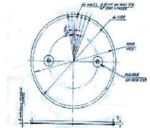
DETAIL OF LID SCALE=1/10
