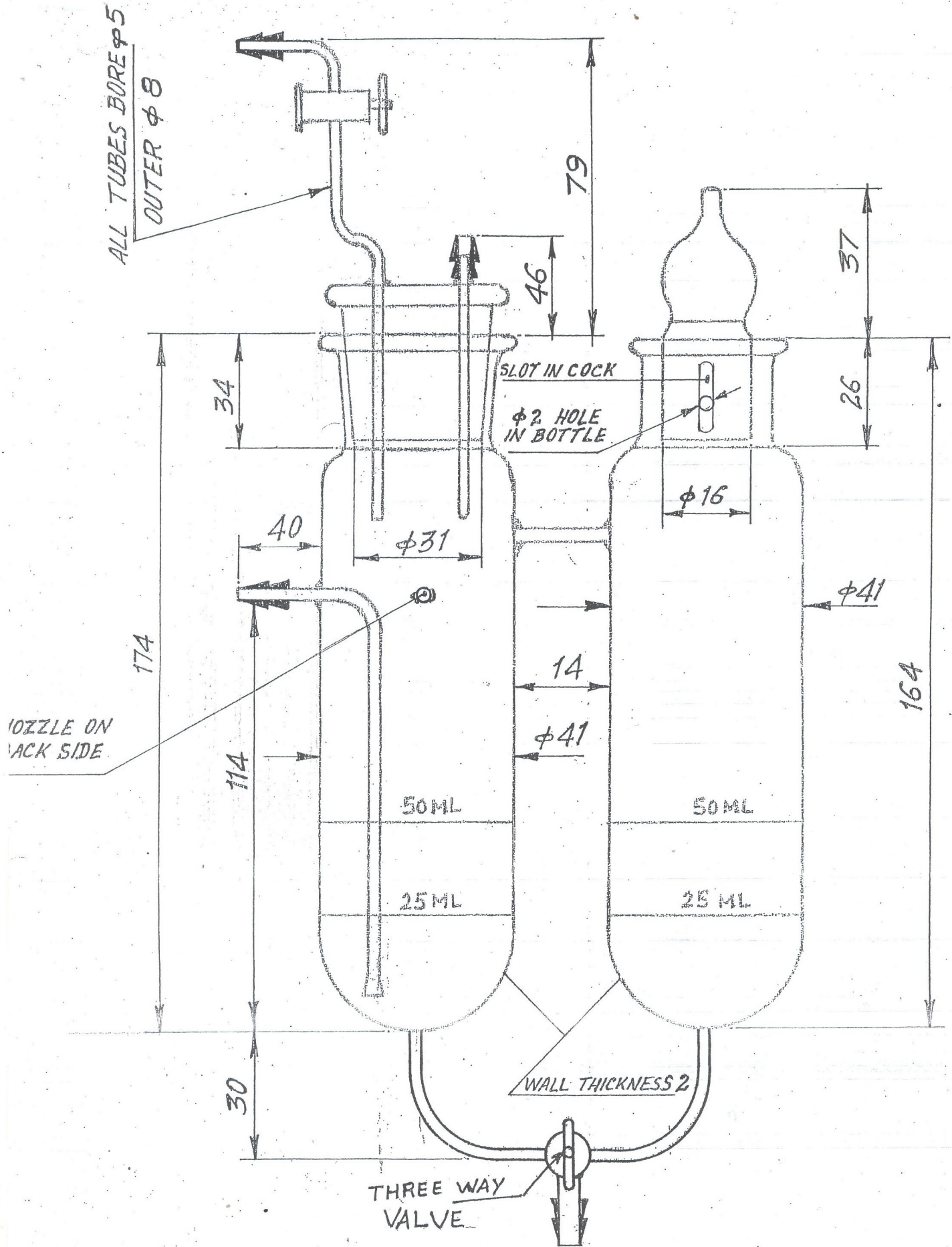
TWIN ABSORPTION BOTTLES (GLASS WARES)
