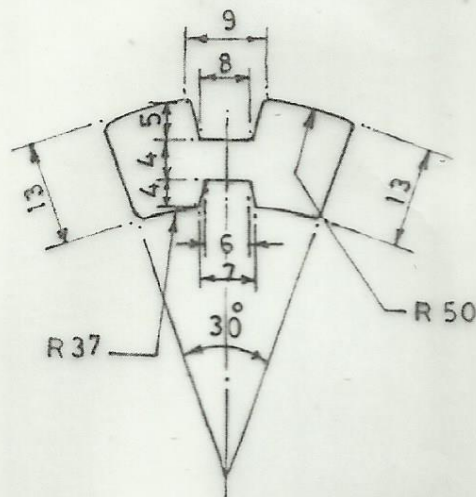
DETAIL OF RUBBER PAD
