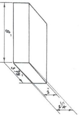
No. 1 ARCH 8 \times 3 \frac{7}{8} " ( 2 \frac{1}{4} \times 2 ")
