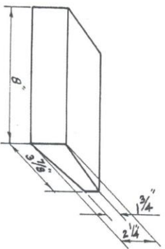
No. 1 WEDGE 8 \times 3 \frac{7}{8} " ( 2 \frac{1}{4} \times 1 \frac{3}{4} ")
